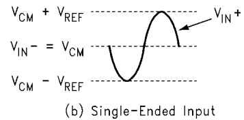
FIGURE 2. Expected Input Signal Range
