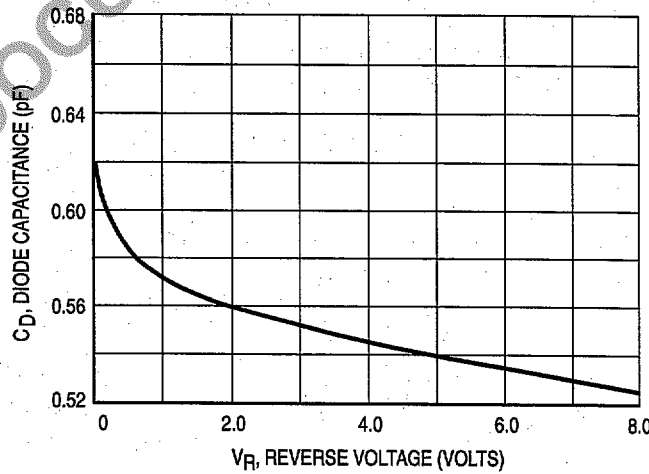
Figure 4. Capacitance
