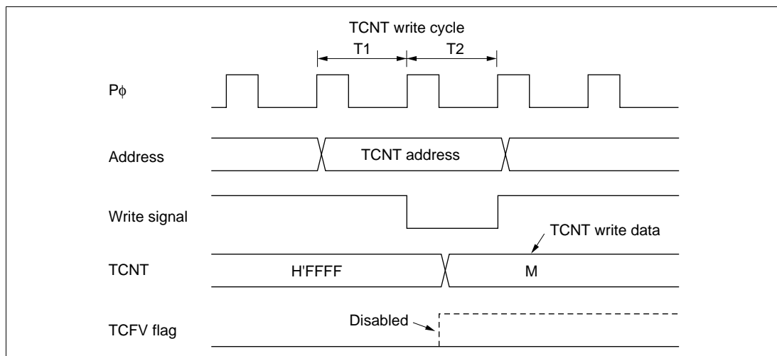
Figure 16.53 Contention between TCNT Write and Overflow
