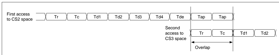
Figure 7.32 Conceptual Diagram of Overlap (Conditions: SDRAM Connected to CS2 Space ( \overline{\text{RAS}} Precharge Time Set to 2 Cycles) and SDRAM Connected to CS3 Space)
