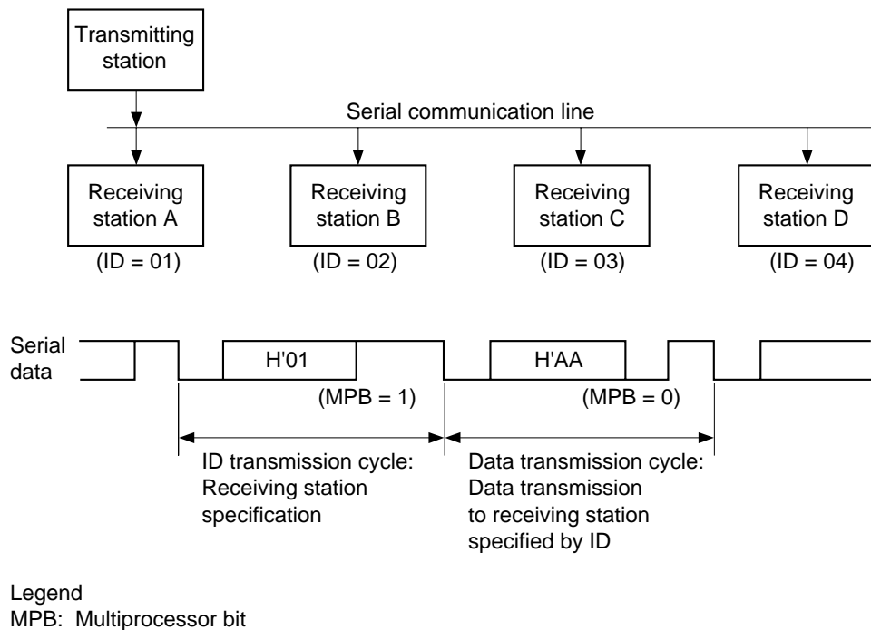
Figure 14.11 Example of Inter-Processor Communication Using Multiprocessor Format (Transmission of Data H'AA to Receiving Station A)
