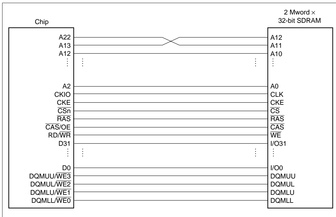
Figure 7.34 64 Mbit Synchronous DRAM (2 Mword × 32 Bit) Connection Example
