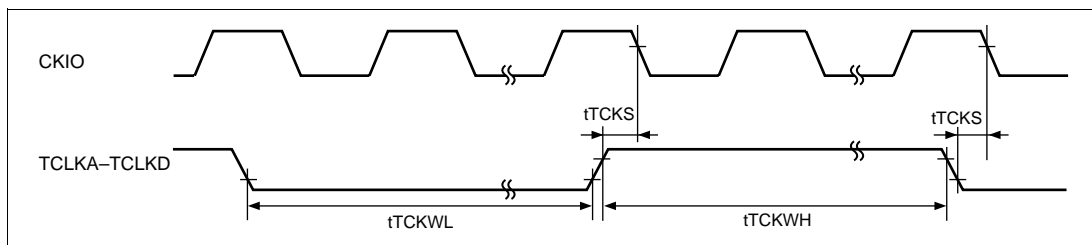
Figure 21.57 TPU Clock Input Timing
