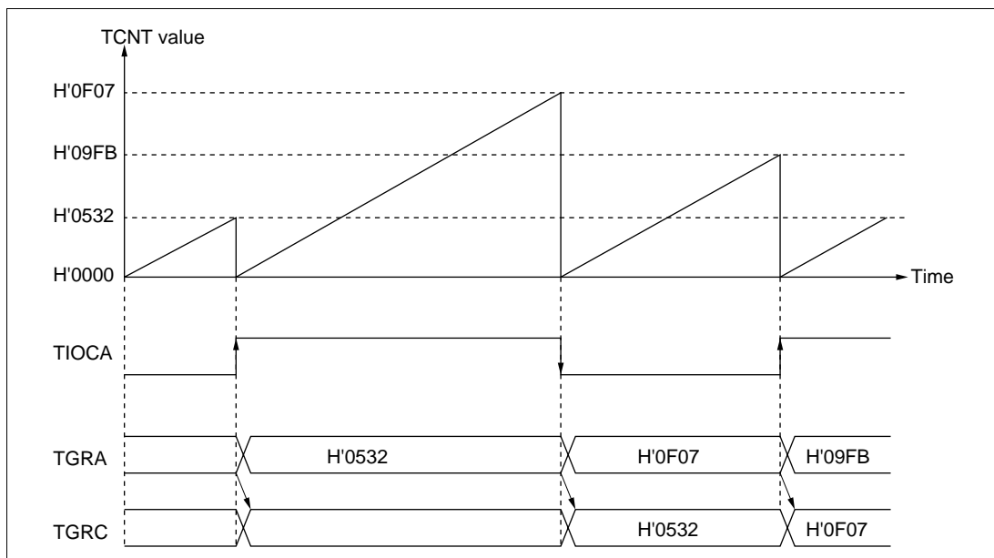
Figure 16.20 Example of Buffer Operation (2)
