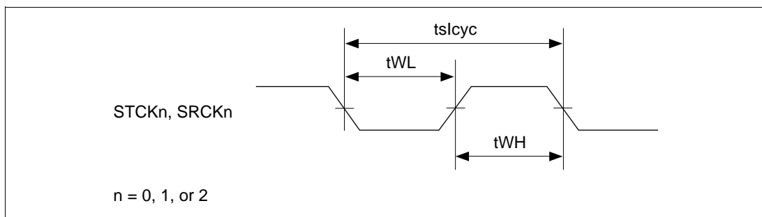
Figure 21.60 SIO Input Clock Timing
