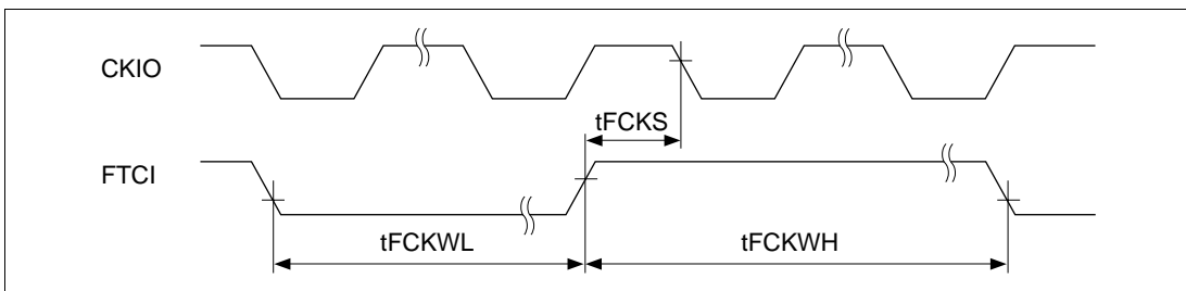
Figure 21.51 FRT Clock Input Timing ( t_{Ecyc}:t_{Pcyc} other than 1:1)
