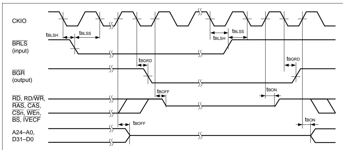
Figure 21.10 Bus Release Timing
