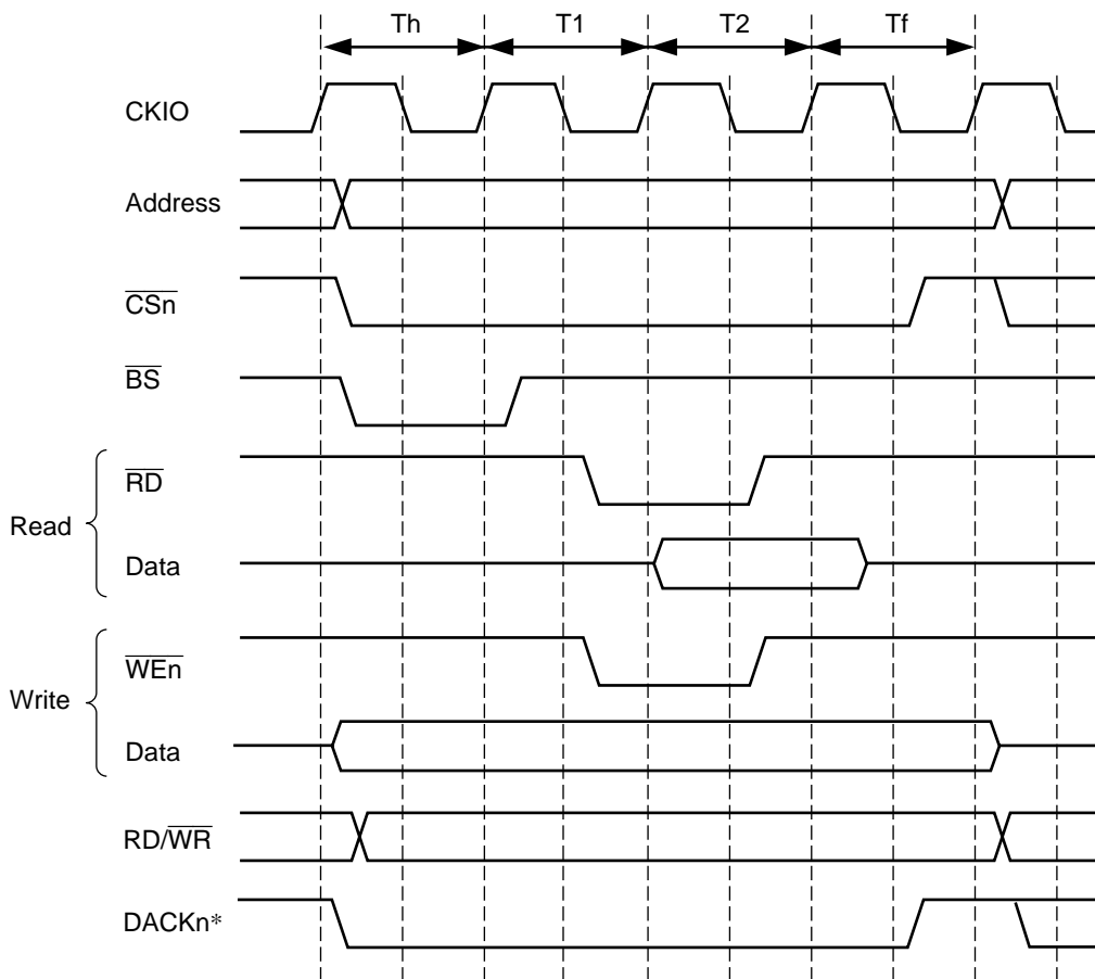
Figure 7.16 \overline{\text{CS}} Assertion Period Extension Function
