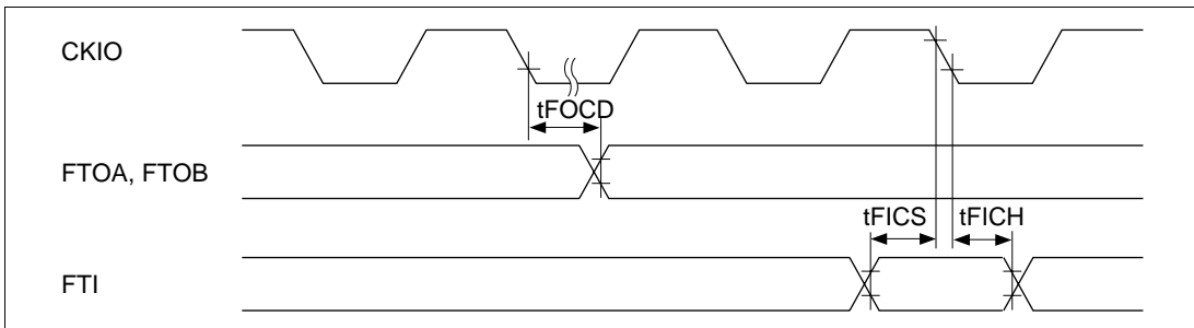
Figure 21.49 FRT Input/Output Timing ( t_{Ecyc}:t_{Pcyc} other than 1:1)
