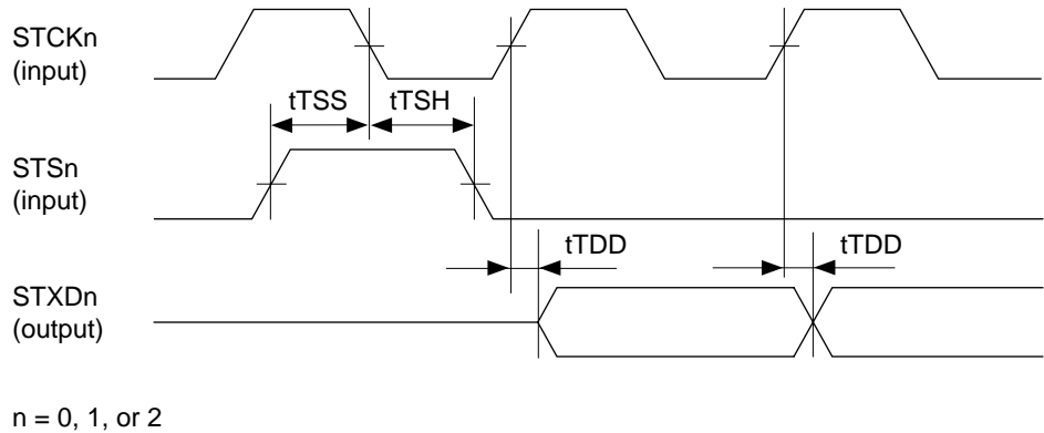
Figure 21.62 SIO Transmit Timing (TMn = 0 Mode)
