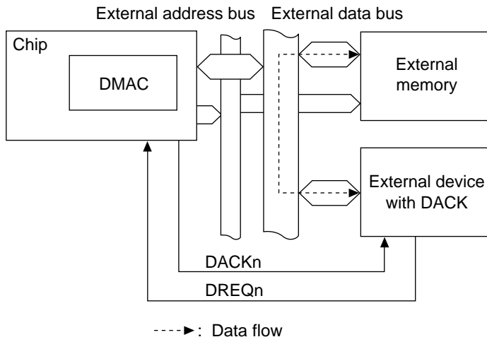
Figure 11.6 Data Flow in Single Address Mode
