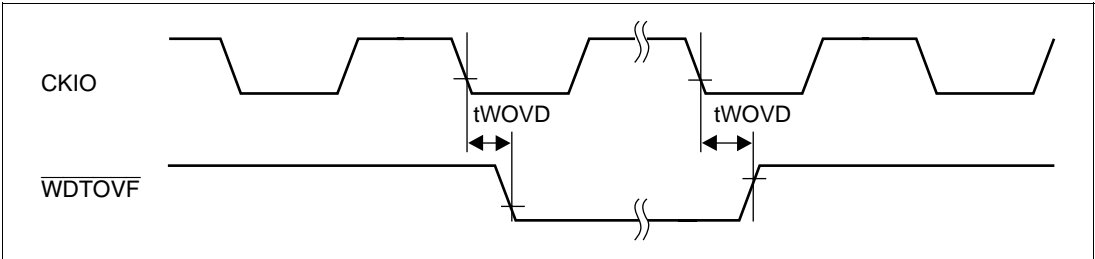
Figure 21.59 Watchdog Timer Output Timing (tEcyc:tPcyc other than 1:1)
