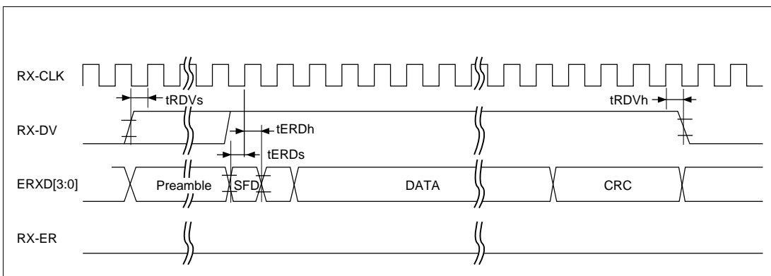
Figure 21.71 MII Receive Timing (Normal Operation)
