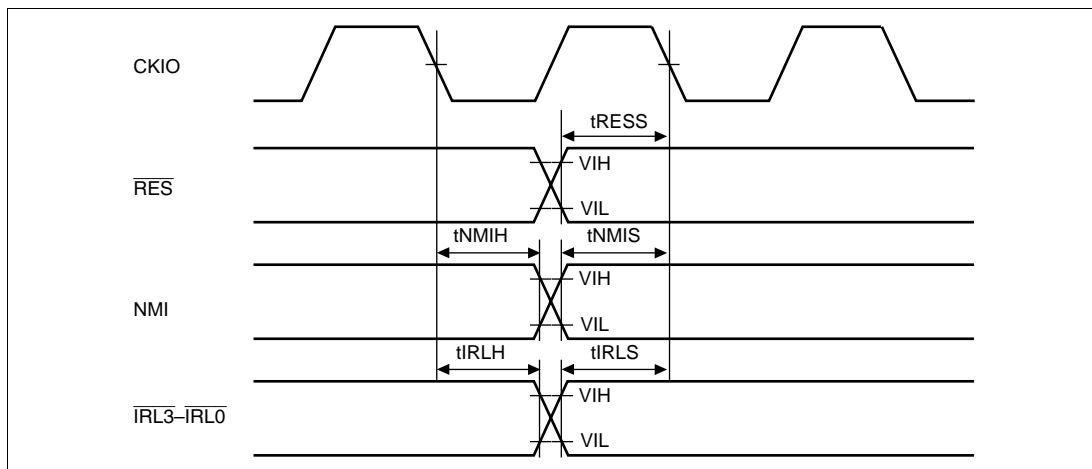
Figure 21.9 Interrupt Signal Input Timing
