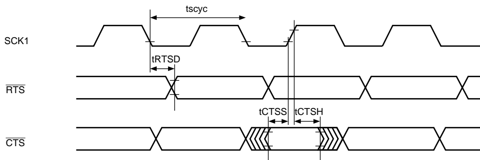
Figure 21.54 \overline{\text{RTS}} and \overline{\text{CTS}} Input/Output Timing
