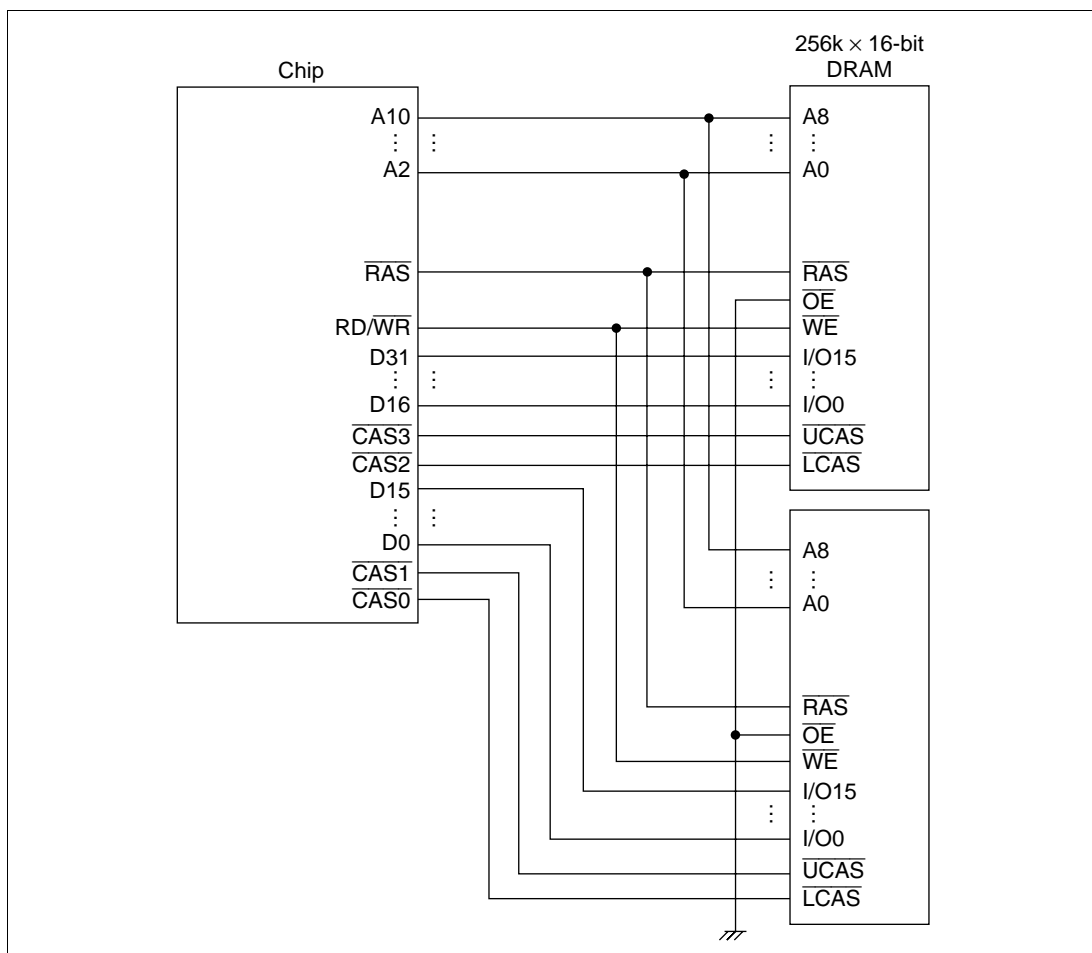
Figure 7.35 Example of DRAM Connection (32-Bit Data Width)
