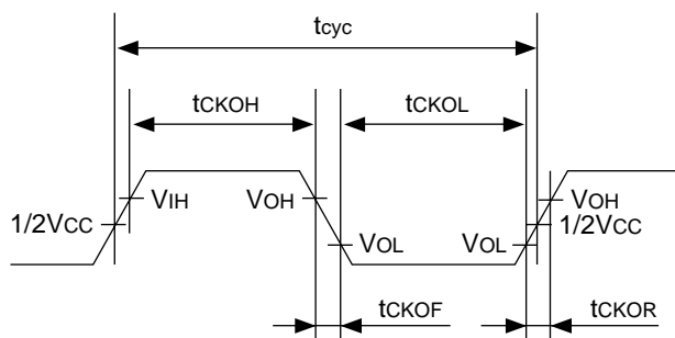
Figure 21.3 CKIO Clock Output Timing
