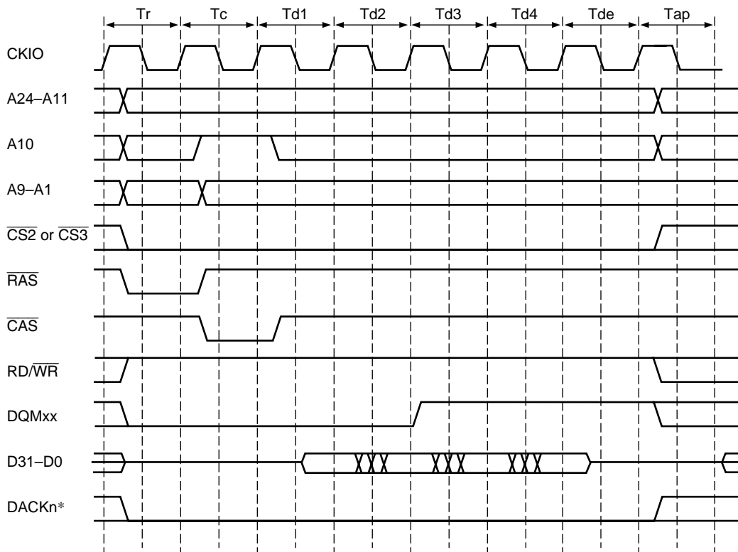
Figure 7.21 (a) Single Read Timing (Auto-Precharge) I\phi : E\phi other than 1 : 1
