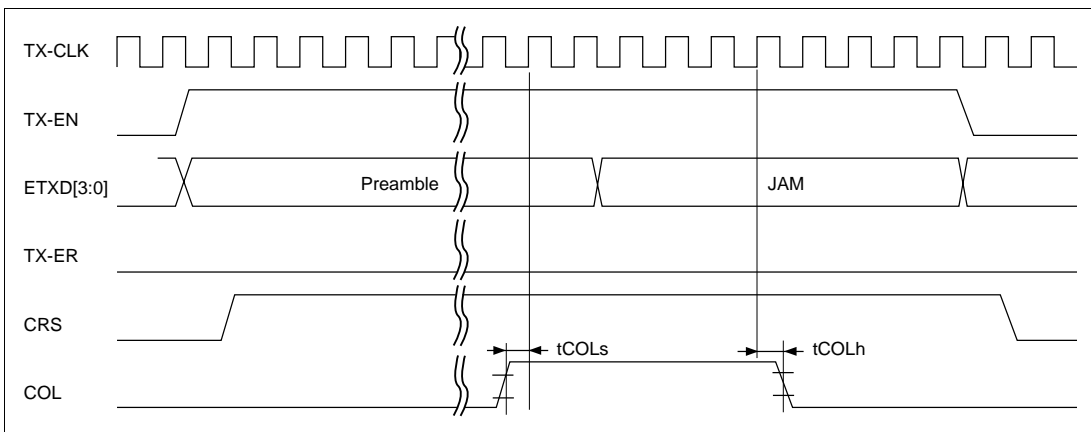
Figure 21.70 MII Send Timing (Case of Conflict)
