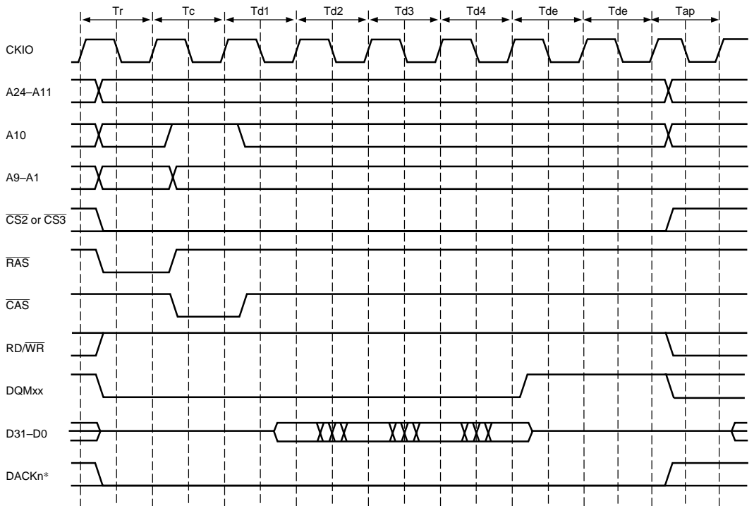
Figure 7.19 (b) Basic Burst Read Timing (Auto-Precharge) I\phi : E\phi = 1 : 1
