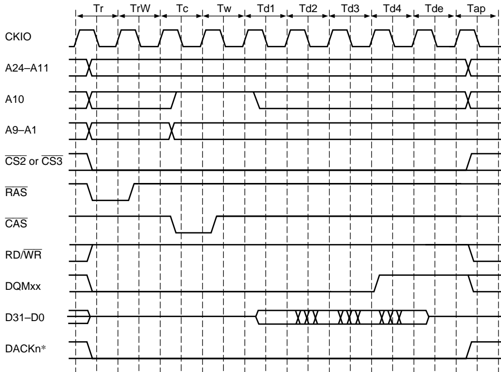
Figure 7.20 (a) Burst Read Wait Specification Timing (Auto-Precharge) I \phi : E \phi other than 1 : 1
