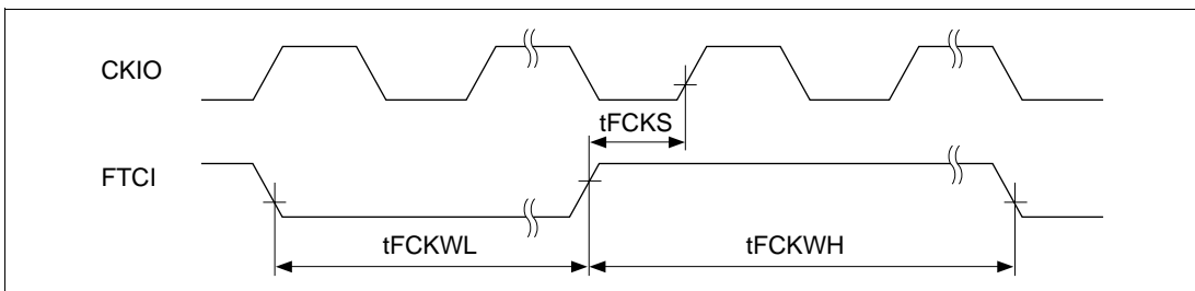
Figure 21.50 FRT Clock Input Timing ( t_{Ecyc}:t_{Pcyc} = 1:1 )
