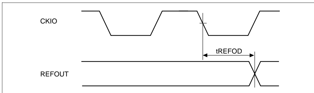
Figure 21.46 REFOUT Delay Time
