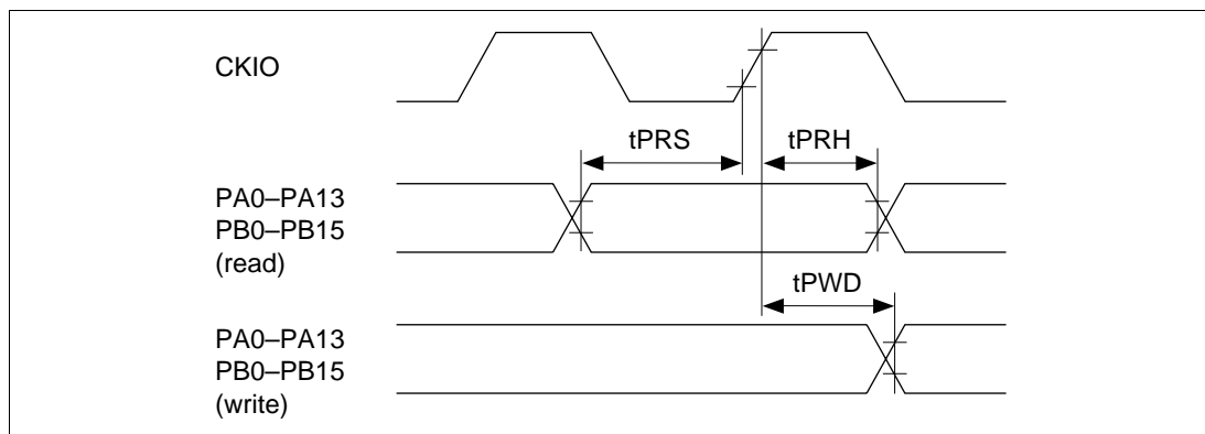
Figure 21.67 I/O Port Input/Output Timing (tEcyc:tPcyc = 1:1)
