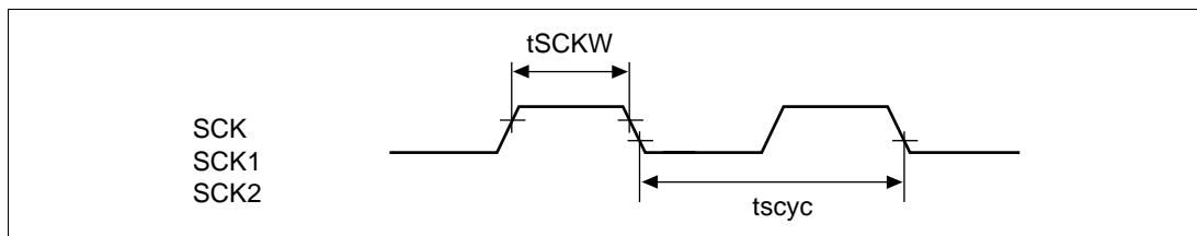
Figure 21.52 Input Clock Input/Output Timing
