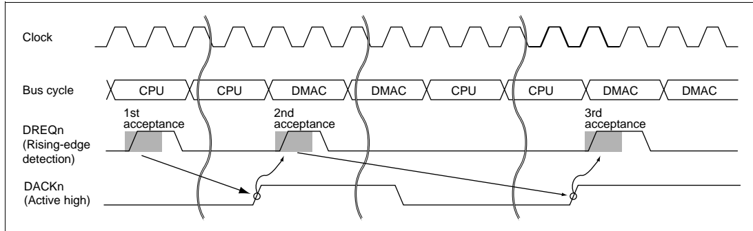
Figure 11.33 DREQn/DACKn Handshaking
