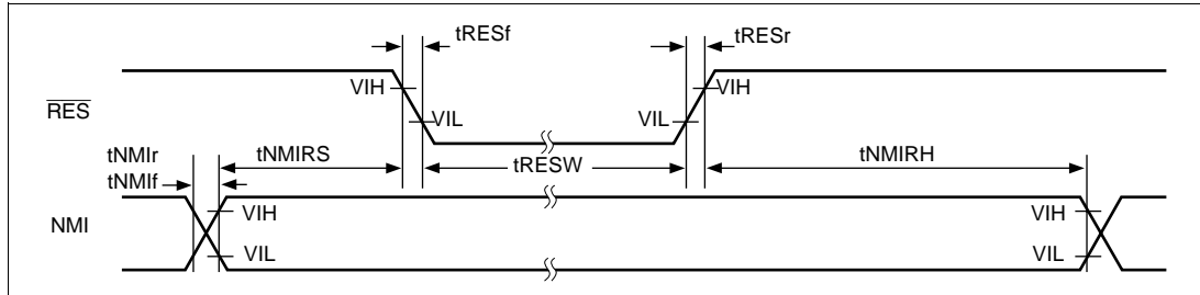
Figure 21.8 Reset Input Timing
