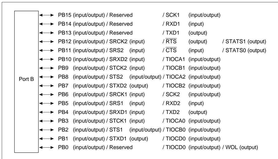
Figure 19.2 Port B
