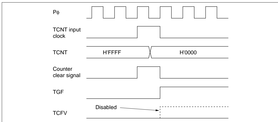
Figure 16.52 Contention between Overflow and Counter Clearing
