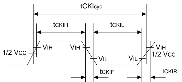
Figure 21.2 CKIO Clock Input Timing
