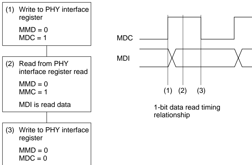
Figure 9.6 (c) 1-Bit Data Read Flowchart
