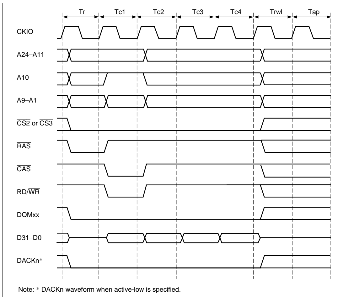
Figure 7.23 (a) Basic Burst Write Timing (Auto-Precharge) Iφ : Eφ other than 1 : 1
