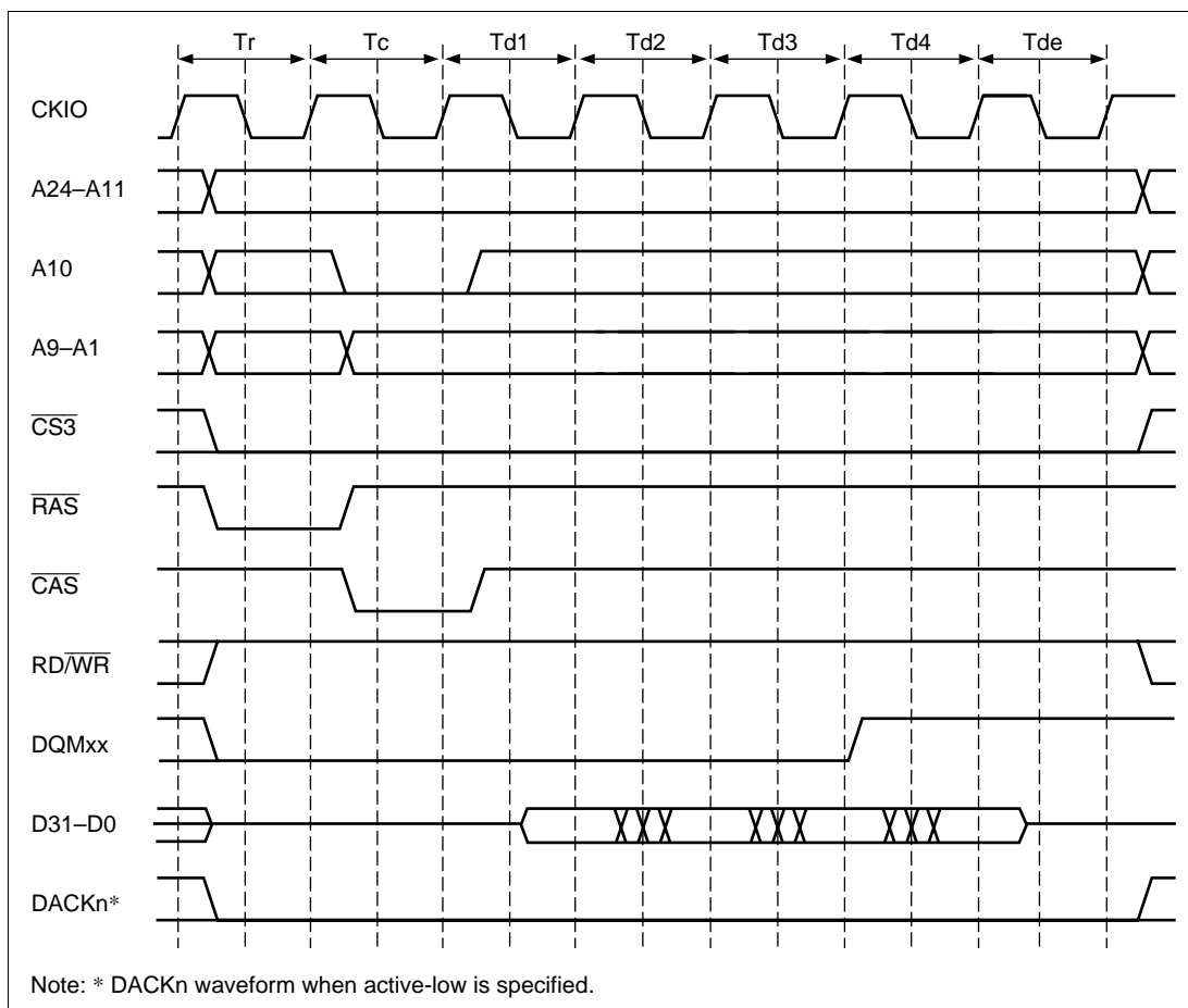
Figure 7.24 (a) Burst Read Timing (No Precharge) I φ : E φ other than 1 : 1
