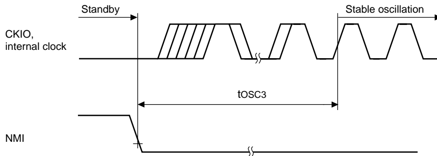
Figure 21.6 Oscillation Stabilization Time after Standby Recovery (Recovery by NMI)
