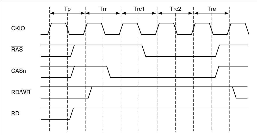
Figure 7.48 DRAM \overline{\text{CAS}} -before- \overline{\text{RAS}} Refresh Cycle Timing
