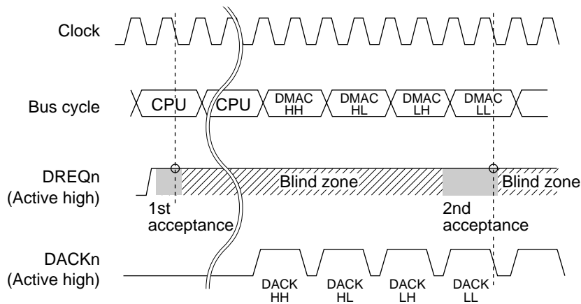
Figure 11.40 When an 8-Bit External Device is Connected (Level Detection)
