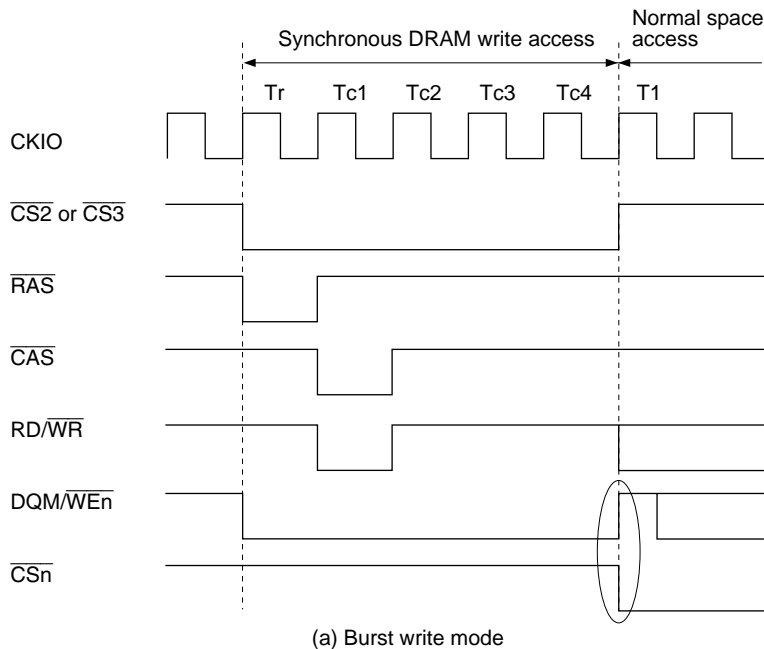
(a) Burst write mode
