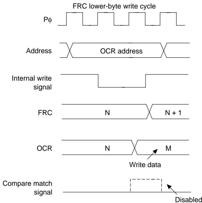
Figure 12.16 Contention between OCR and Compare Match
