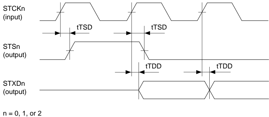
Figure 21.63 SIO Transmit Timing (TMn = 1 Mode)
