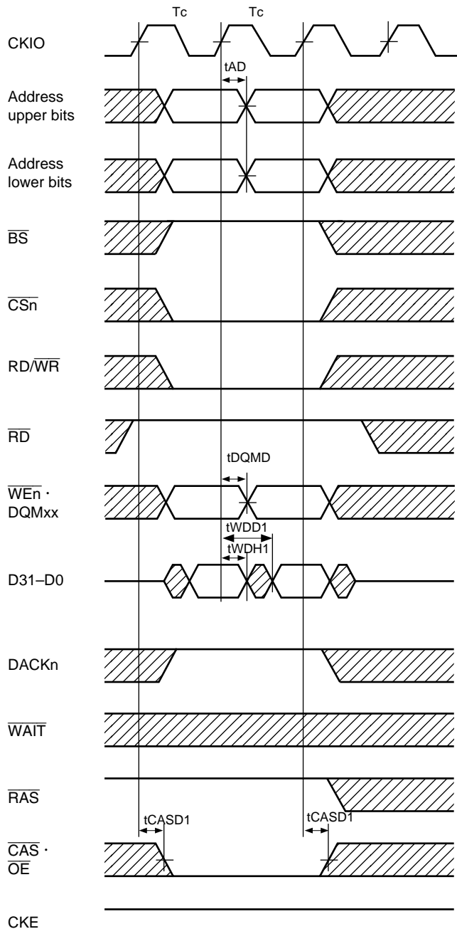
Figure 21.26 Synchronous DRAM Continuous Write Cycle (Bank Active, Same Row Access, I\phi:E\phi other than 1:1)
