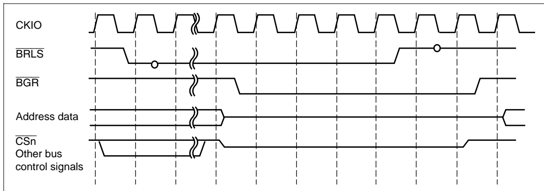
Figure 7.55 Bus Arbitration
