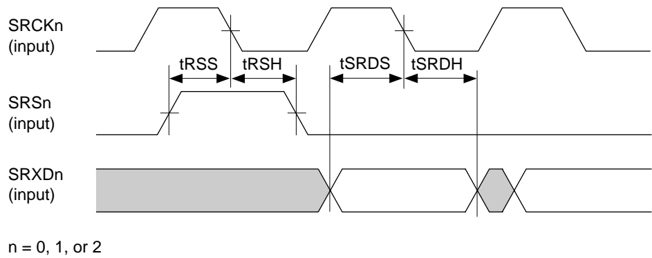
Figure 21.61 SIO Receive Timing
