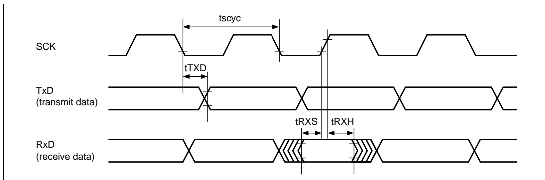
Figure 21.53 SCI Input/Output Timing (Synchronous Mode)
