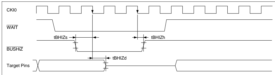
Figure 21.79 BUSHiZ Bus Timing
