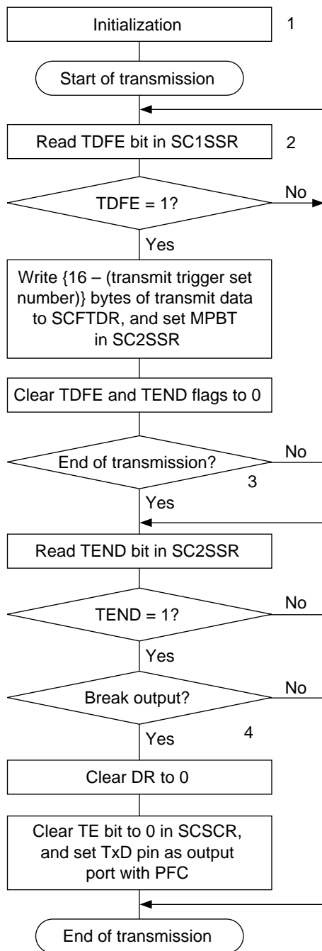
Figure 14.12 Sample Multiprocessor Serial Transmission Flowchart
