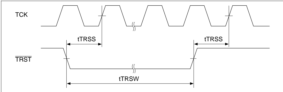
Figure 21.65 H-UDI \overline{\text{TRST}} Timing
