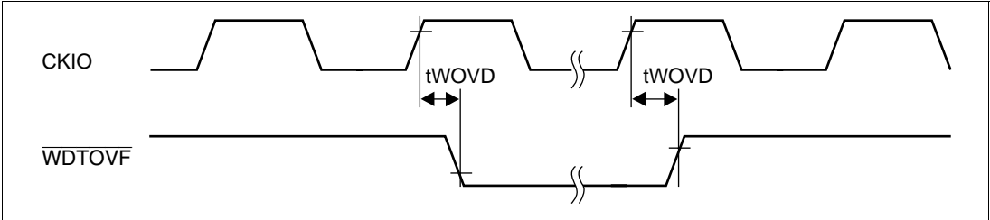
Figure 21.58 Watchdog Timer Output Timing (tEcyc:tPcyc = 1:1)
