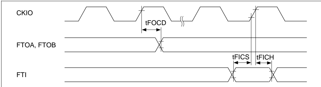
Figure 21.48 FRT Input/Output Timing ( t_{Ecyc}:t_{Pcyc} = 1:1 )
