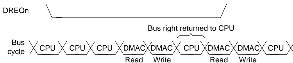
Figure 11.10 DMA Transfer Timing in Cycle-Steal Mode (Dual Address Mode, DREQn Low Level Detection)
