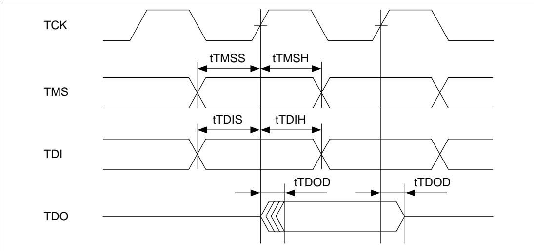
Figure 21.66 H-UDI Input/Output Timing
