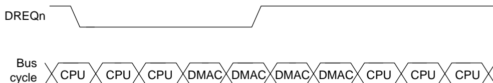
Figure 11.11 DMA Transfer Timing in Burst Mode (Single Address, DREQn Falling-Edge Detection)
