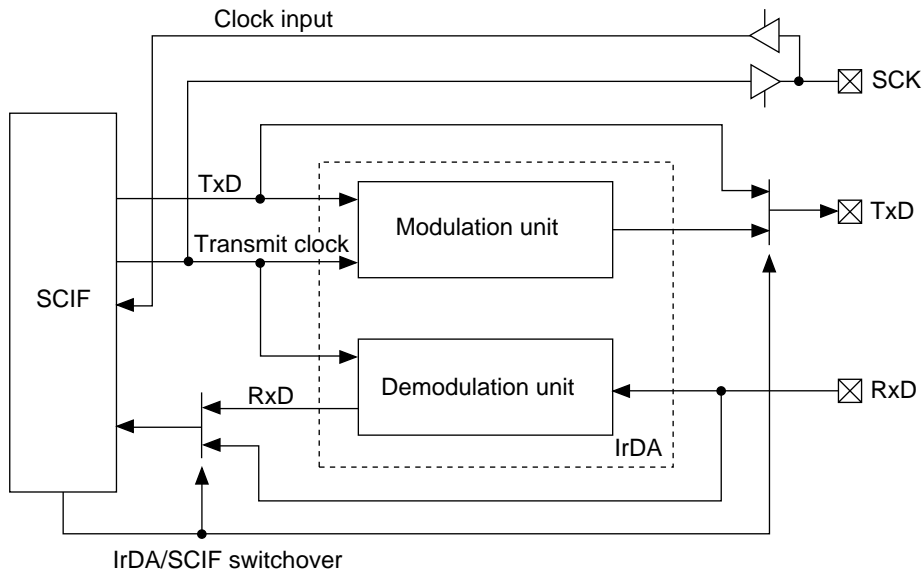
Figure 14.2 Diagram of IrDA Block
