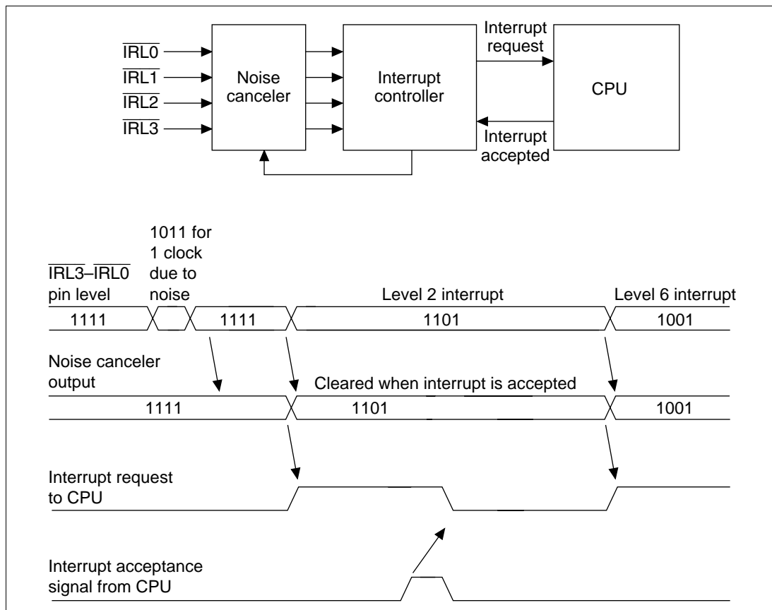
Figure 5.10 \overline{\text{IRL3}} – \overline{\text{IRL0}} Pin Sampling
